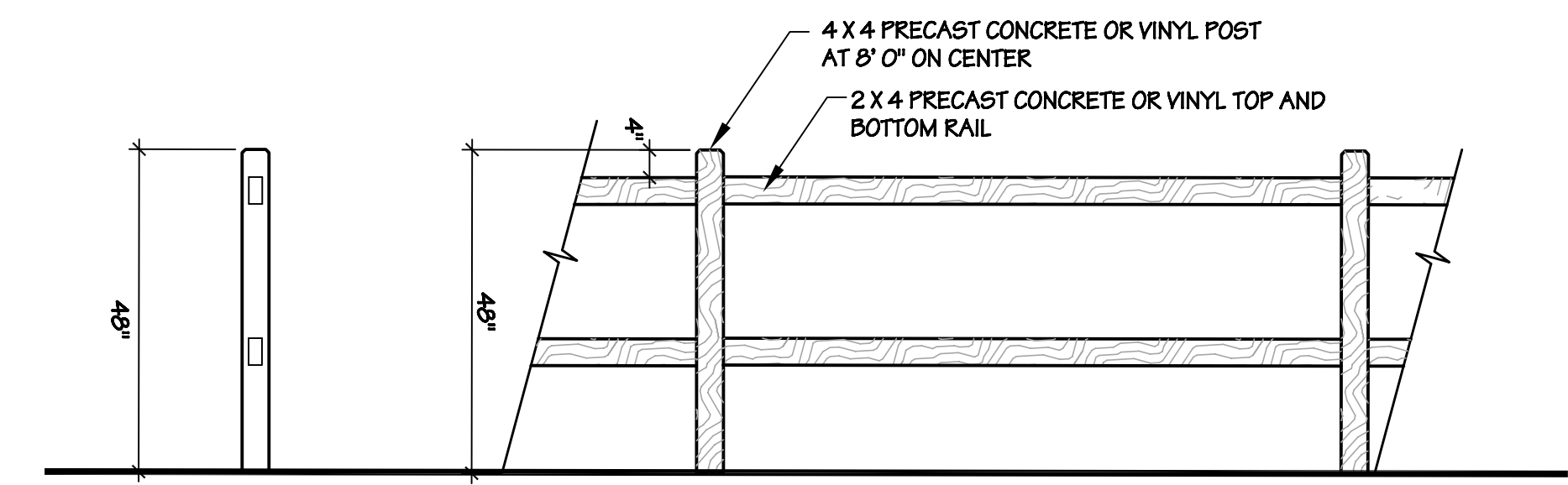
C 48" HIGH SPLIT RAIL FENCE SCALE: NOT TO SCALE
