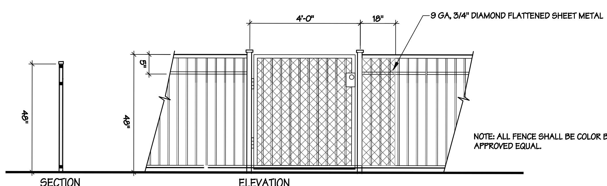
B 48" HIGH PAINTED TUBULAR STEEL FENCE AND GATE SCALE: NOT TO SCALE
