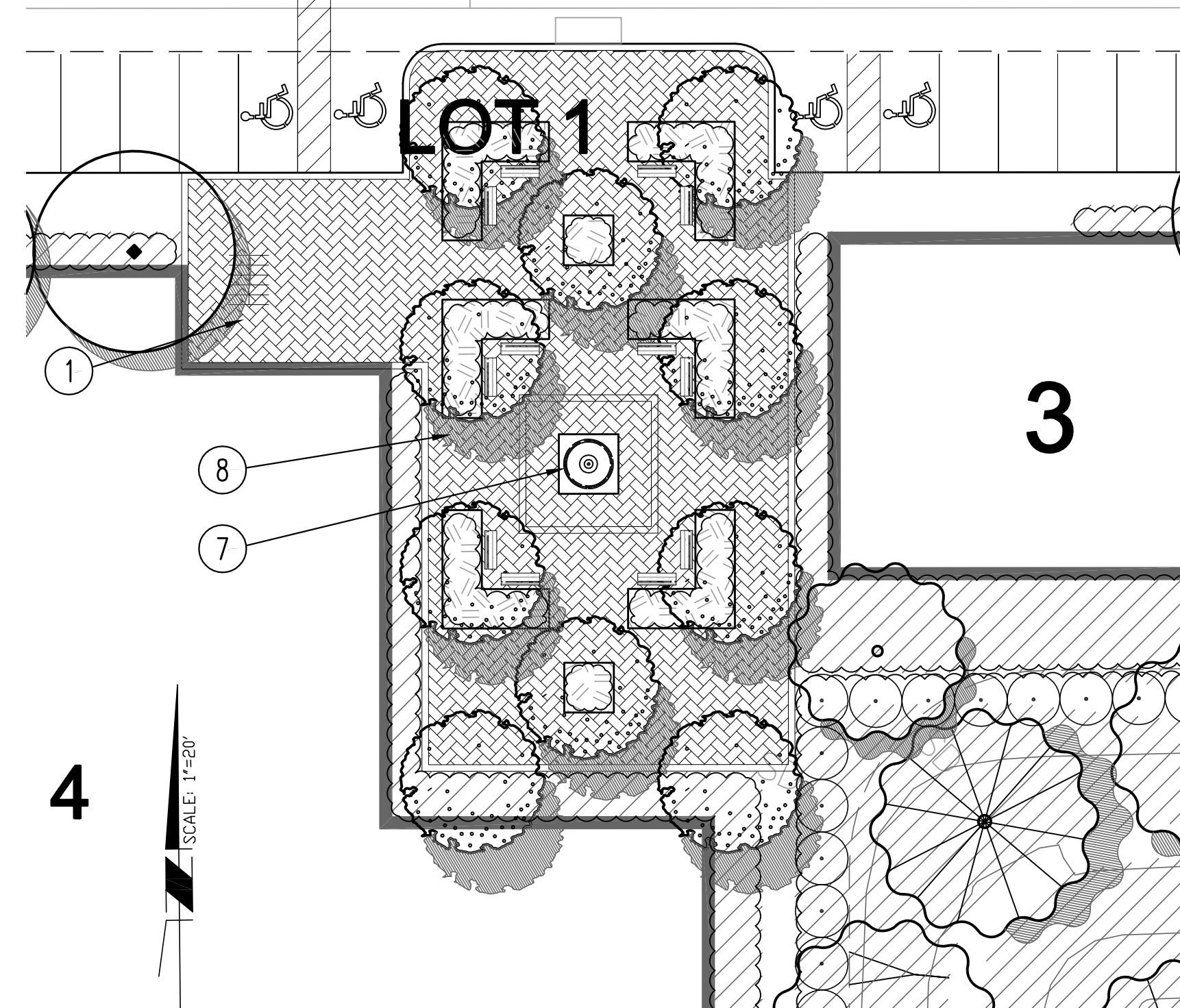
A ENHANCED ENTRY LANDSCAPE AND MOUNMENT AT CLINTON KEITH ROAD AND PEDESTRIAN PLAZA SCALE: 1" = 20'-0"
