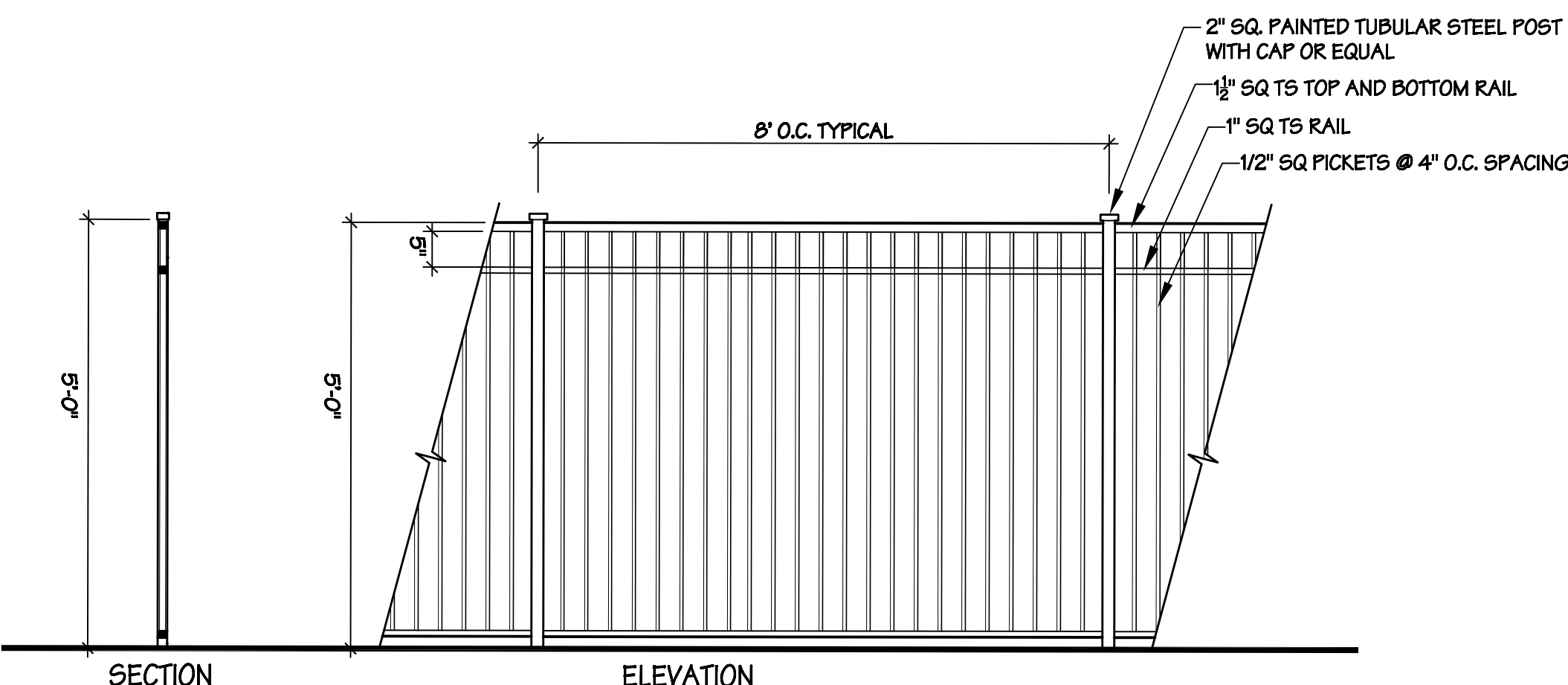
A 5' HIGH PAINTED TUBULAR STEEL FENCE SCALE: NOT TO SCALE
